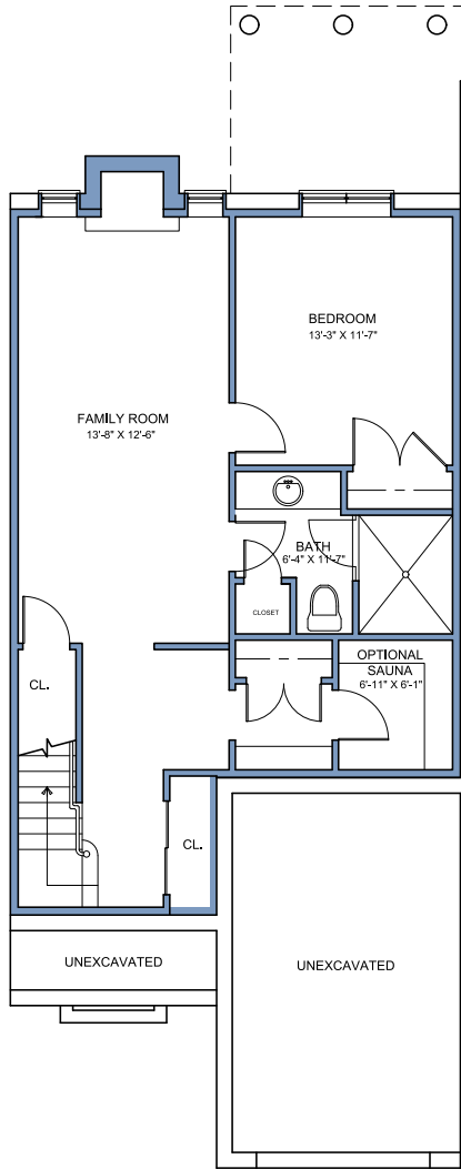
GROUND LEVEL
