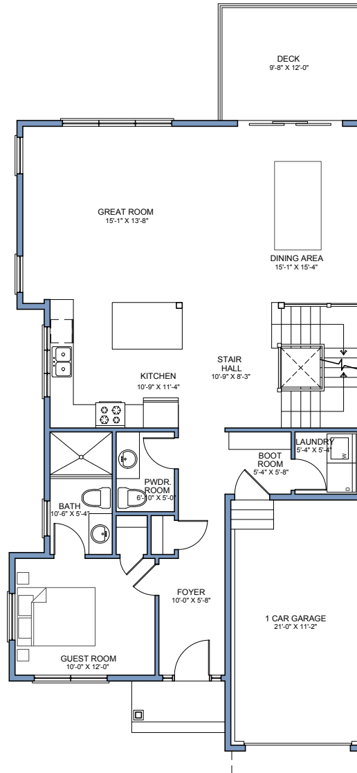
FIRST FLOOR
